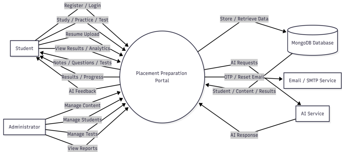
Figure 5.2.1 DFD Level 0
