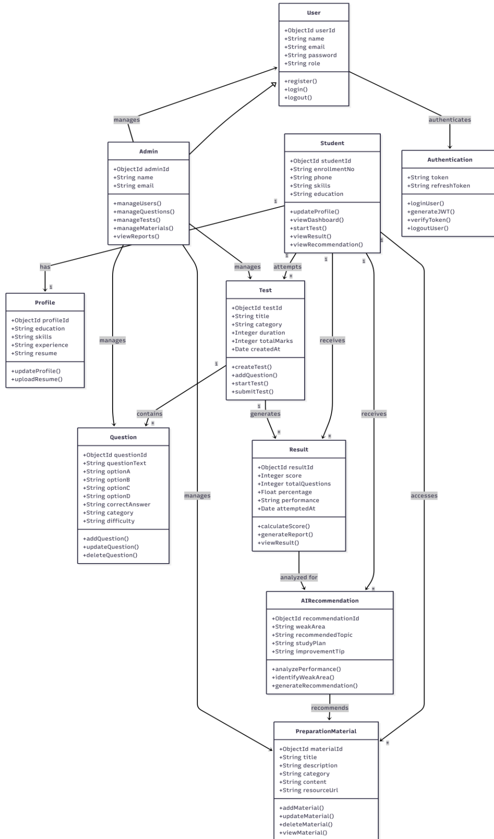
Figure 5.5 Class Diagram
