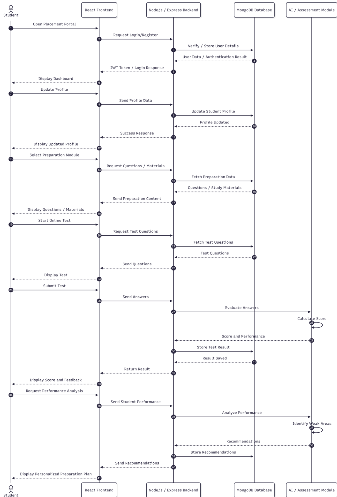
Figure 5.4 Sequential Diagram
