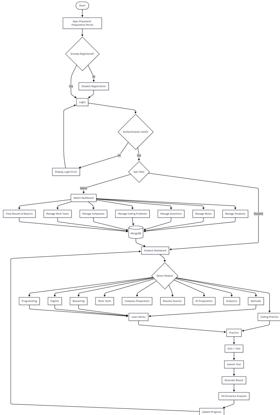
Figure 5.1 Flow Chart
