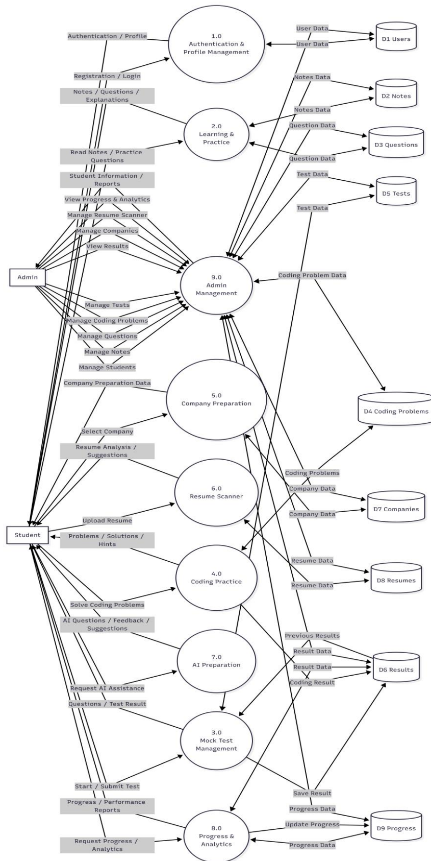
Figure 5.2.2 DFD Level 1
