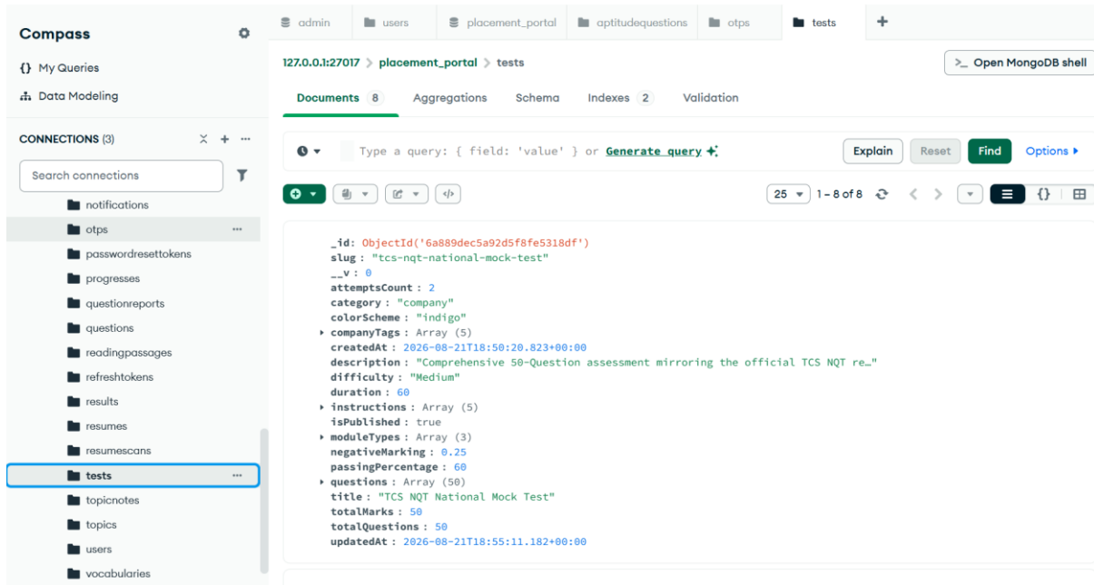
Figure 5.7.15 Test
